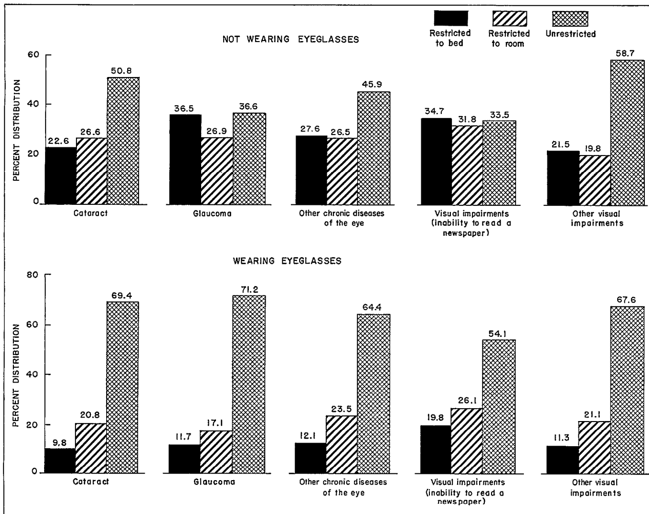
Figure 4. Percent distribution of residents with specified eye diseases and impairments, by mobility status according to whether eyeglasses were worn.
