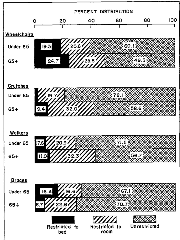
Figure 5. Percent distribution of residents using specified special aids, by age according to mobility status.
