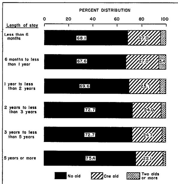
Figure 2. Percent distribution of residents, by number of special aids used (excluding hearing aids and eyeglasses) according to length of stay.
