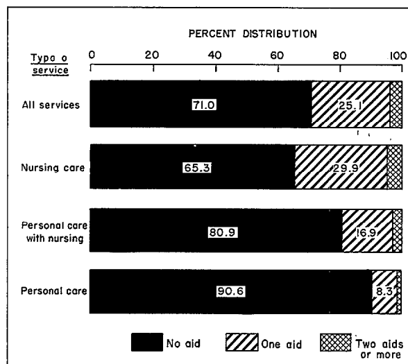
Figure 1. Percent distribution of residents, by number of special aids used (excluding hearing aids and eye-glasses) according to type of service.
