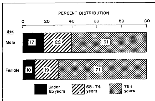
Figure 3. Percent distribution of residents using wheelchairs, by age according to sex.
