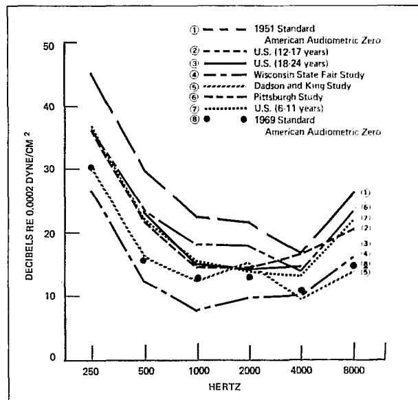
Figure 16. Median hearing threshold levels for right ear (in decibels re 0.0002 dynes per cm 2 ) for youths and young adults at selected frequencies, from selected studies.
