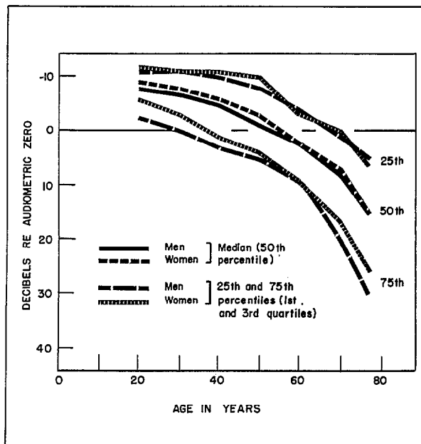
Figure 8. Medians and quartiles from the distribution of the hearing threshold levels for speech (average of pure-tone levels at 500, 1000, and 2000 cycles per second) in the better ear for men and women, United States.
