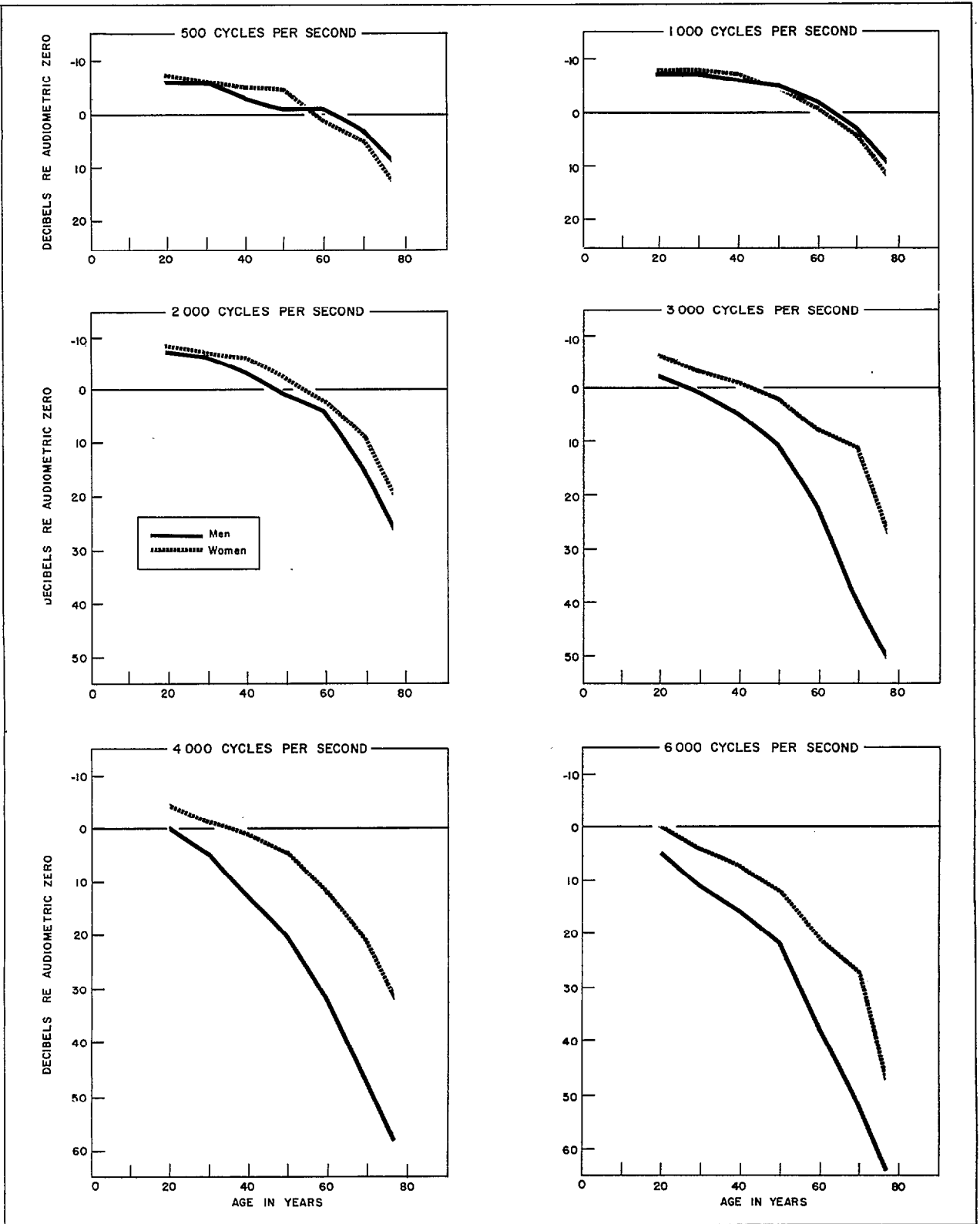
Figure 7. Median hearing levels for the better ear of men and women, by age at each test frequency, United States.
