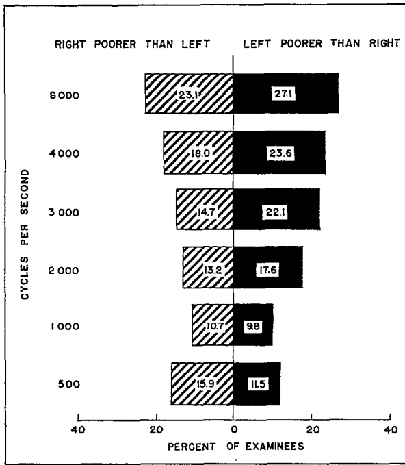
Figure 4. Percent with hearing levels in the two ears differing by more than 5 decibels, Health Examination Survey.
