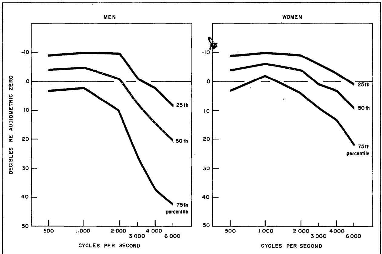
Figure 6. Medians and quartiles (50th, 25th, and 75th percentiles) from the distribution of hearing threshold levels for the better ear of men and women 18-79 years of age at six frequencies, United States.
