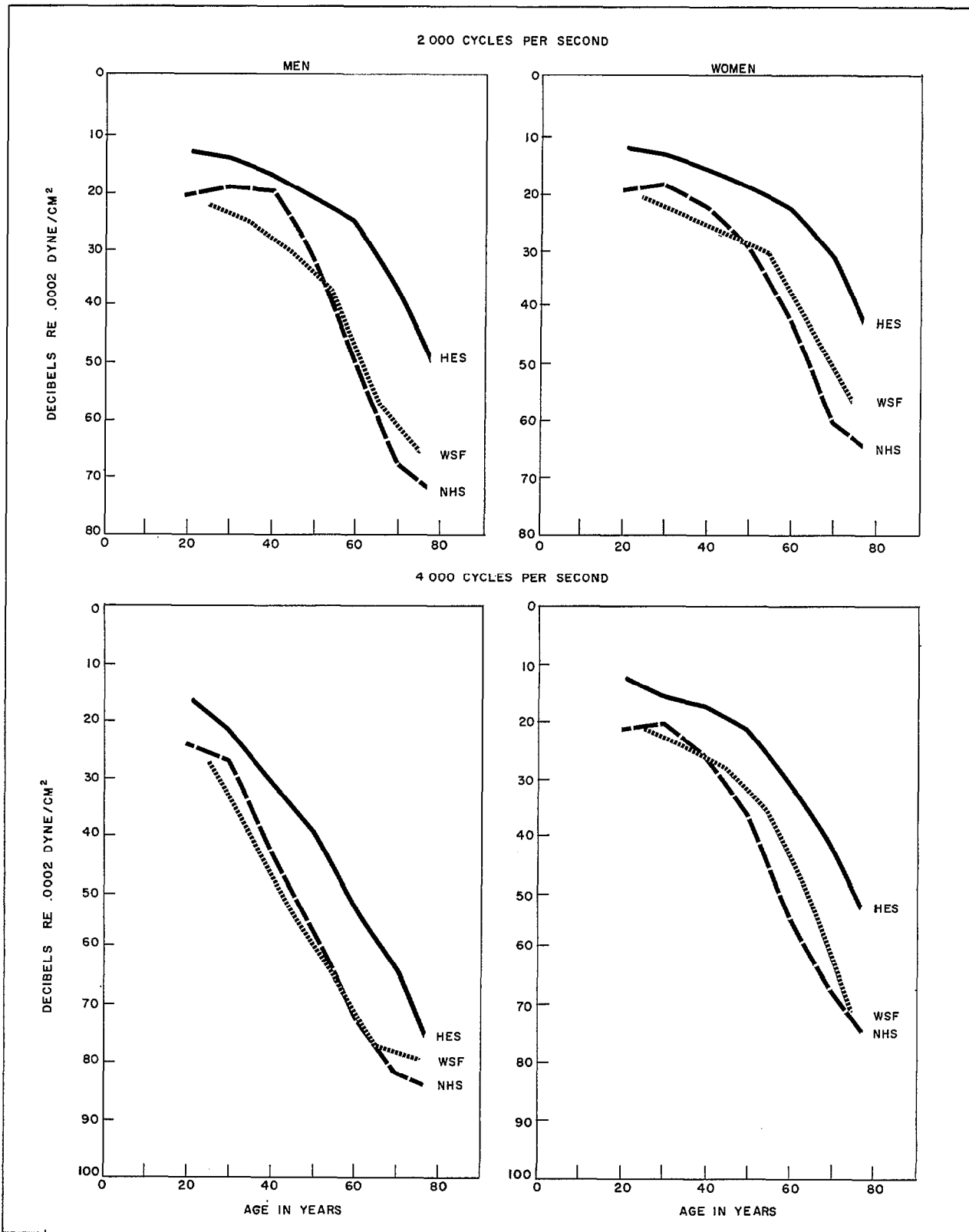
Figure 9. Median hearing threshold levels (in decibels re 0.0002 dyne per square centimeter) for men and women, by age at four frequencies, from the present study, the 1964 Wisconsin State Fair Survey, and the 1935-36 National Health Survey —Con.
