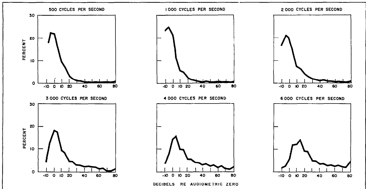
Figure 3. Percent distribution of hearing levels for adults at each test frequency, Health Examination Survey.
