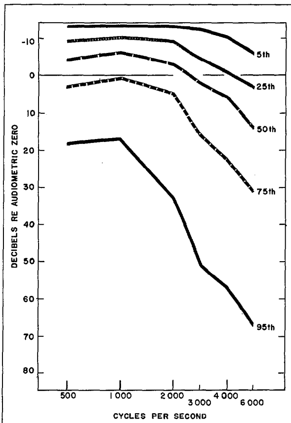
Figure 2. Selected percentiles from the distribution of hearing threshold levels for the better ear of adults at each test frequency, United States.
