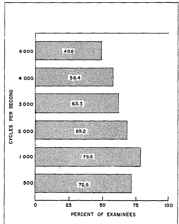
Figure 3. Percent with difference in hearing levels between both ears of 5 decibels or less, Health Examination Survey.
