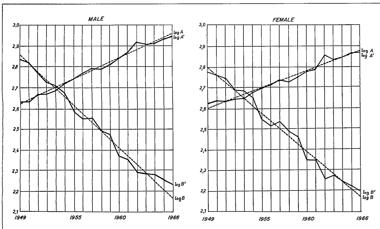
Figure 11. Linear interpolation of the logarithms of the components A , B of the death rate for males and for females: Czech regions, 1949-66.
