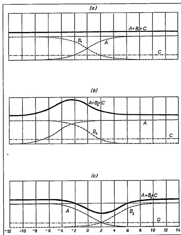
Figure 10. Mathematical models of trends in heterogeneous populations II.
