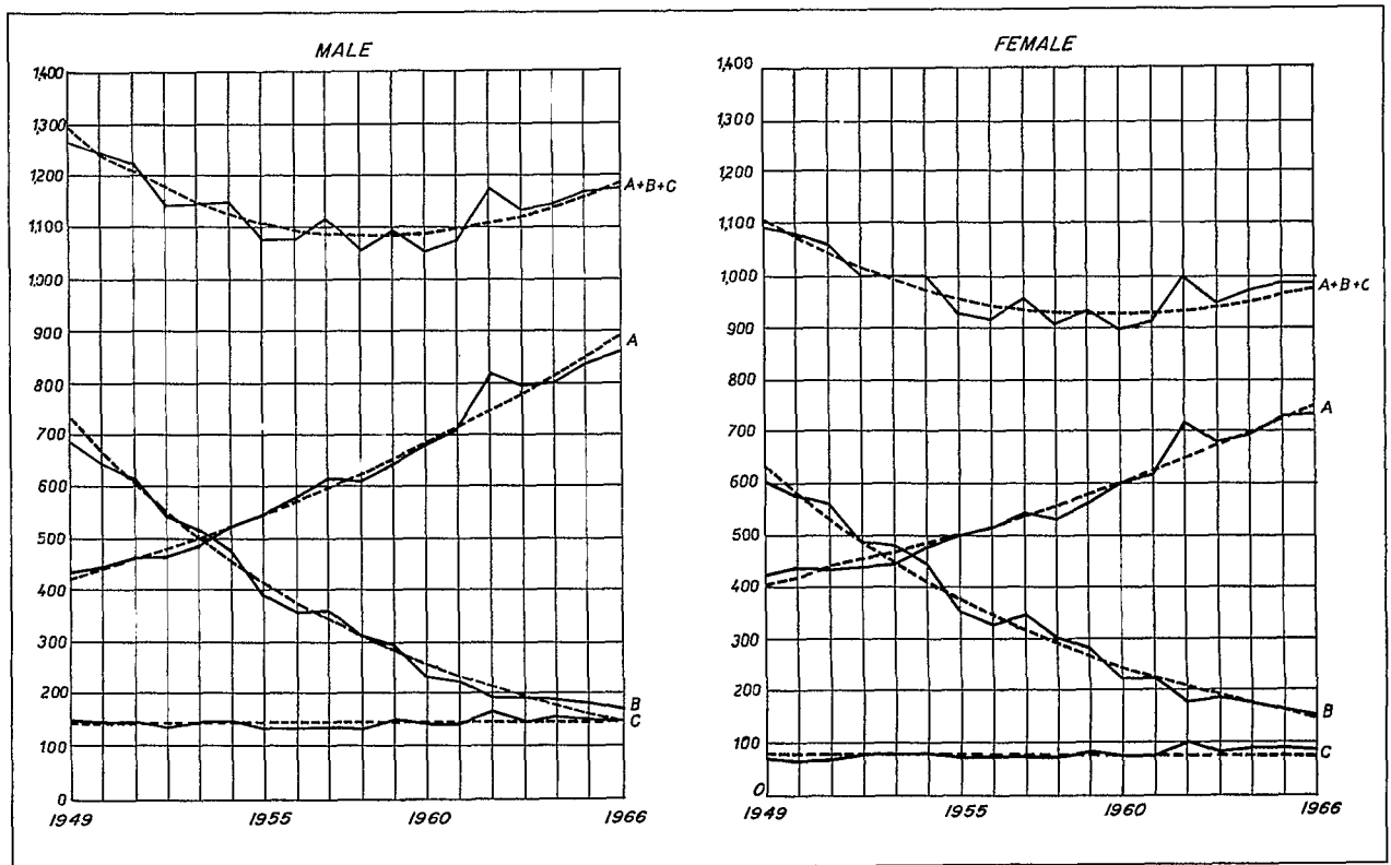
Figure 12. Breakdown of the crude death rate for males and for females into three components: Czech regions, 1949-66.
