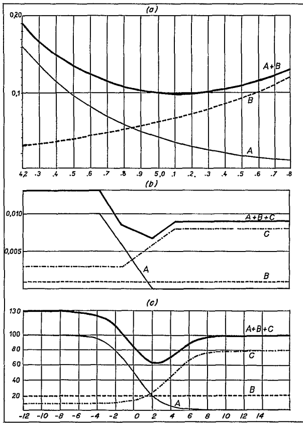
Figure 9. Mathematical models of trends in heterogeneous populations I.
