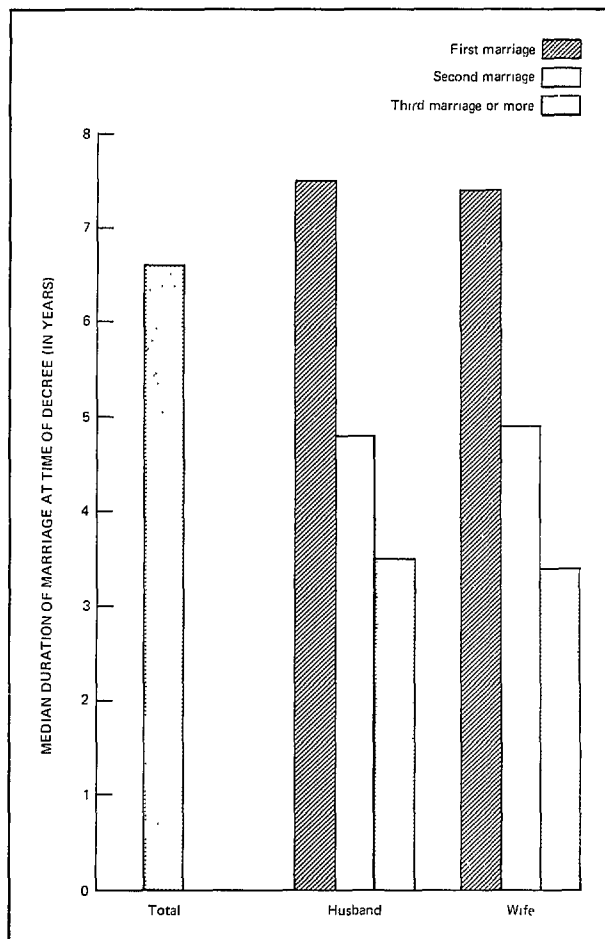
Figure 6. Median duration of marriage at time of decree by number of this marriage of husband and wife: Divorce-registration area, 1977
