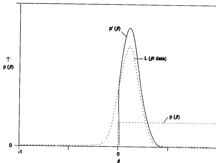
Figure A-2. Schematic of computing a posterior distribution [p'(\beta^C)] from a likelihood function [L(\beta | \text{data})] and a prior distribution [p(\beta)] .
