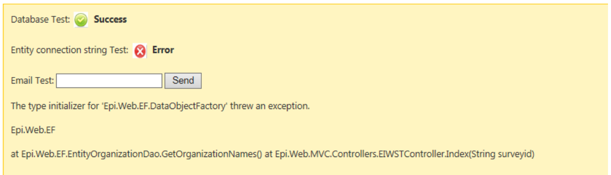
Figure 33: Epi Info™ Cloud Data Capture diagnostics view showing status when the application can communicate with the database server, but an error exists with the connection string.
