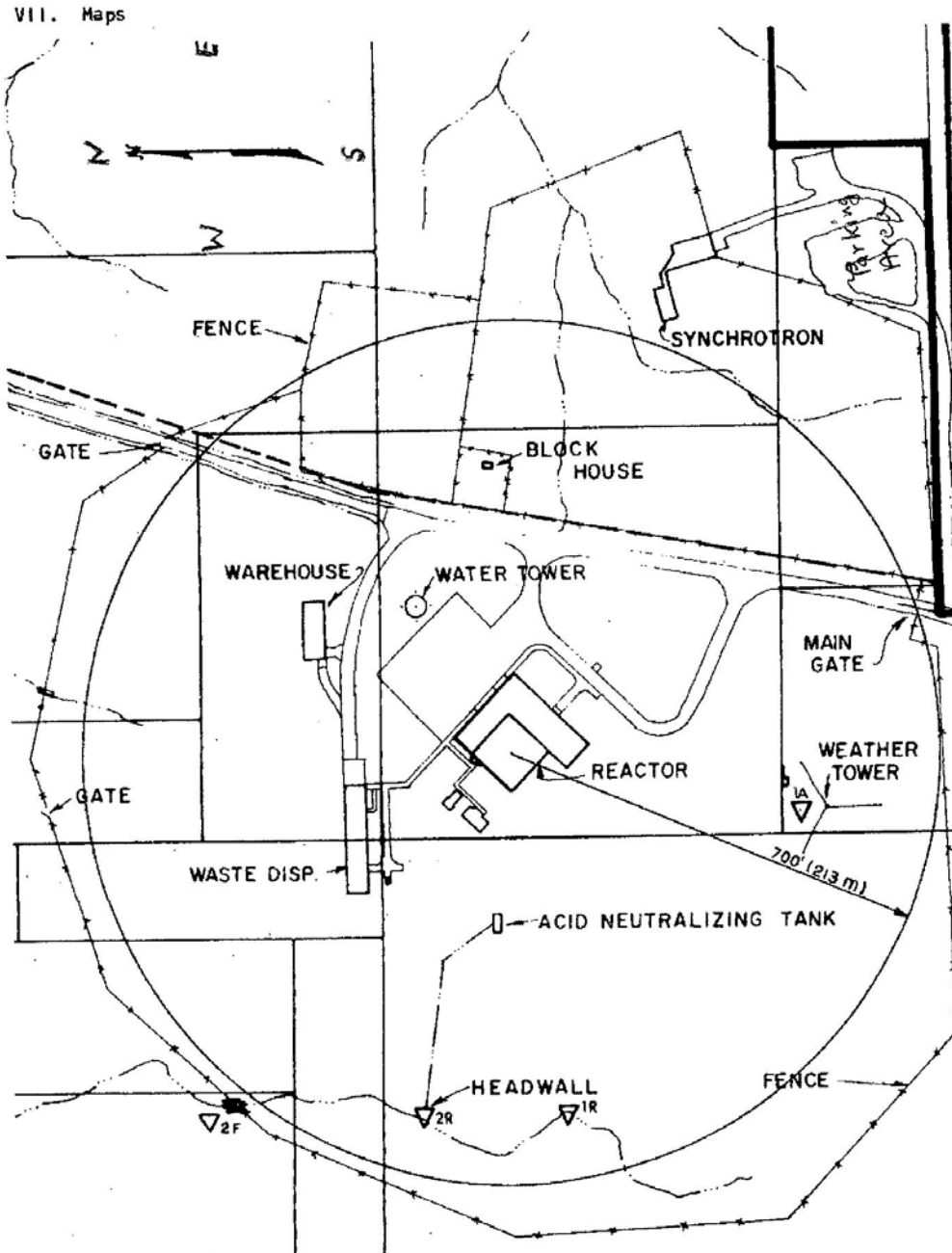
Figure 1: Ames Laboratory Research Reactor Site Plan. Map drawn to scale.
