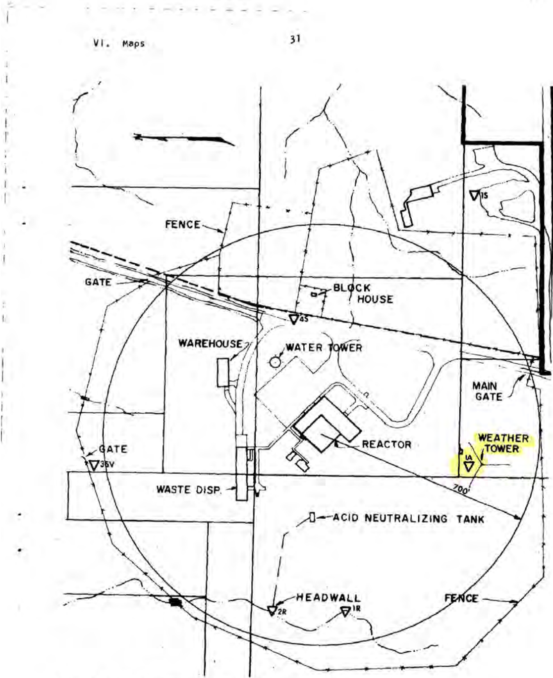
Figure 1: Ames Laboratory Research Reactor Site Plan. Map drawn to scale.
