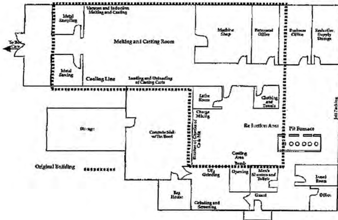
Figure 1. Floor Plan of Little Ankeny Production Facility for Uranium and Thorium
