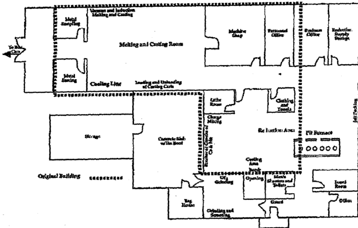
Figure 3-3. Floor Plan of Little Ankeny Production Facility for Uranium and Thorium (Note: Heavy dotted line identified original buildings.)
