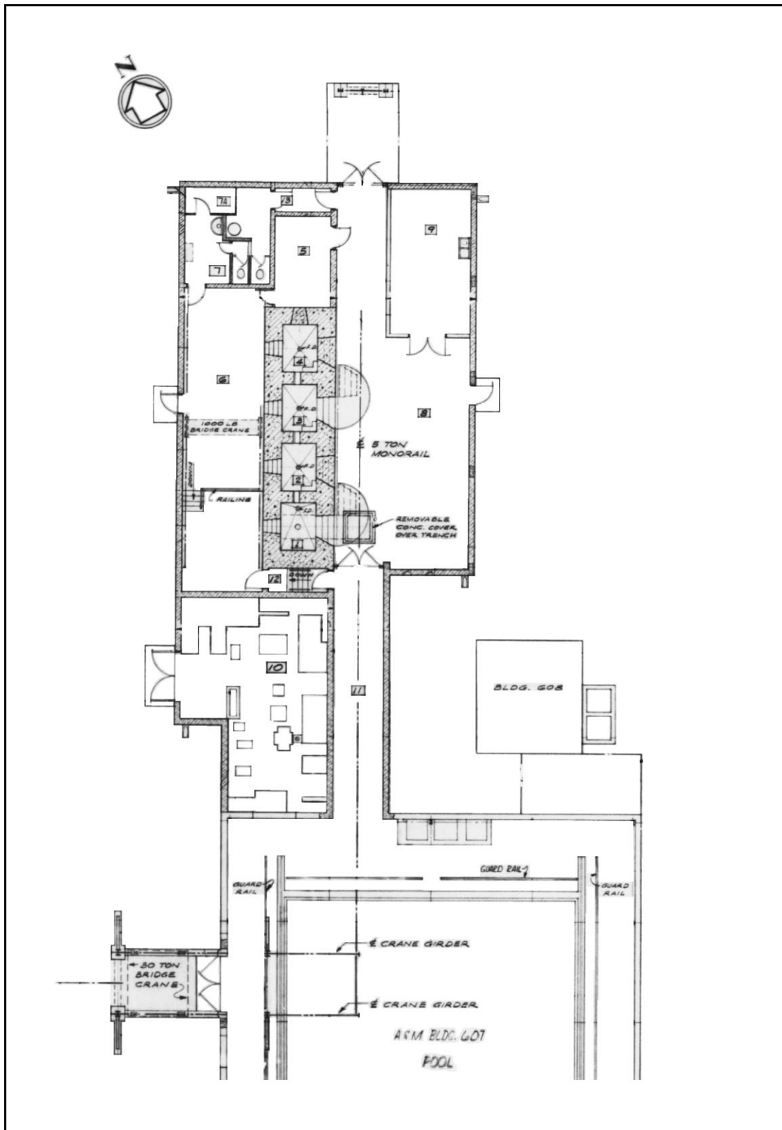
Figure 5-33: Floor Plan of Hot Cell Annex (TAN-633)
