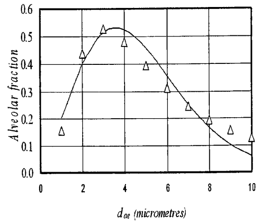
Fig. 11 Calculated results for alveolar deposition efficiency as a function of particle aerodynamic diameter ( d_{ae} ) for mouth breathing by a 'reference worker' from the model of James et al. , 17 also shown is the curve describing the proposed new criterion for the alveolar deposition fraction (open triangles).
