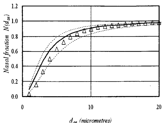
Fig. 9 Calculated results for nasal deposition efficiency as a function of particle aerodynamic diameter ( d_{ae} ) for relatively low Q -values of 10, 20 and 30 L \text{ min}^{-1} (continuous and dashed lines) from the model of James et al. 17 also shown is the curve describing the proposed new criterion for the nasal fraction (open triangles).
