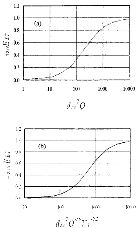
Fig. 4 Efficiency of extrathoracic deposition ( E_{ET} ): (a) for nasal deposition (mainly in the anterior region) following nose breathing; 16,20-22 and (b) head deposition (mainly in the larynx) following mouth breathing. 21,23,24 The data are plotted as functions of combinations of variables suggested by James et al. 17 The shaded areas represent the experimental data and the continuous curves are calculated from the models proposed by James et al.
