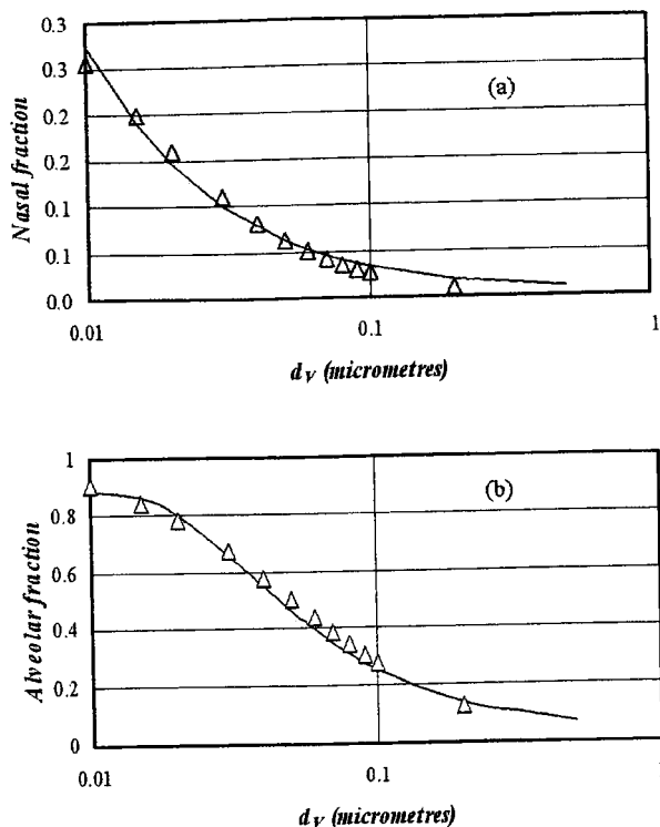
Fig. 12 Calculated results for nasal and alveolar deposition efficiency as a function of particle equivalent volume diameter ( d_v ) for ultrafine particles from the models of James et al. 17 also shown are the curves for the proposed new criteria for the nasal and alveolar deposition fractions (open triangles).
