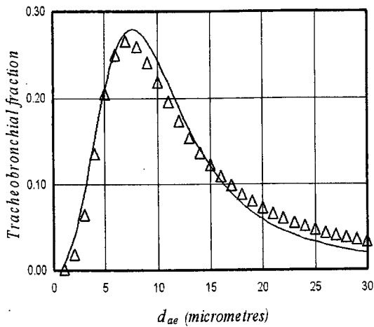
Fig. 10 Calculated results for tracheobronchial deposition efficiency as a function of particle aerodynamic diameter ( d_{ae} ) for mouth breathing by a 'reference worker' from the model of James et al. , 17 also shown is the curve describing the proposed new criterion for the tracheobronchial fraction (open triangles).
